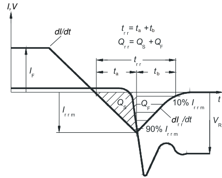
Figure C. Definition of diodes switching characteristics
