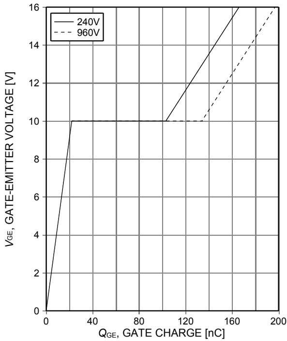
Figure 17. Typical gate charge ( I_C=40A )
